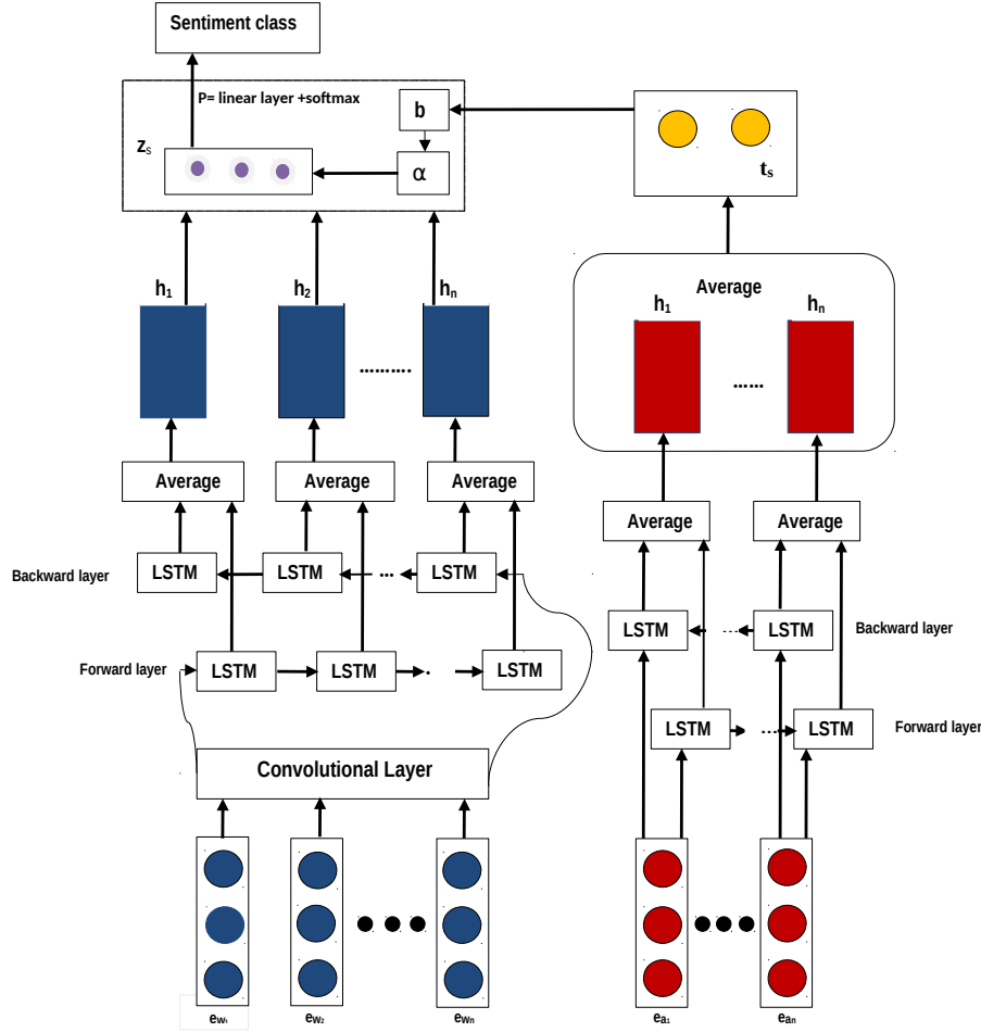
Figure 1: CNN-BiLSTM framework for aspect sentiment classification
